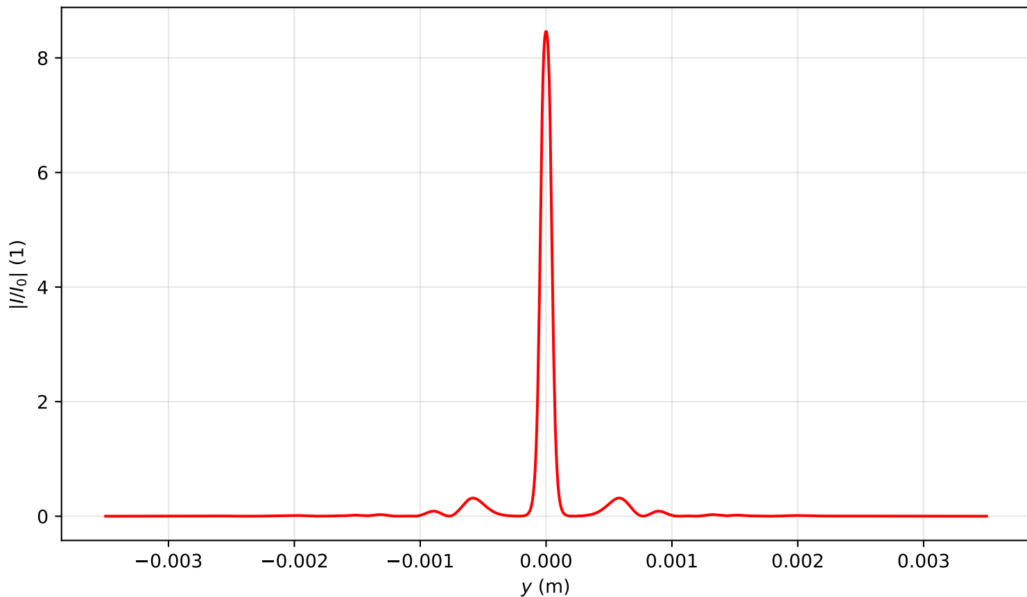
Intensity profile I(x = 0, y, z = 0.478)/I_0 , P_{in}=8.0P_{cr} , artificial time
